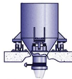
IP 67 Double Ended shear beam load cell with Tank mounting kit.
